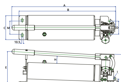
HP 35 model
